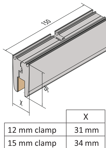
Glass Clamp Dimension
