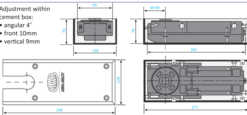
Single action doors / offset Right
