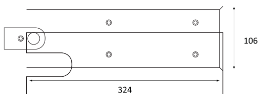
Cover plates
